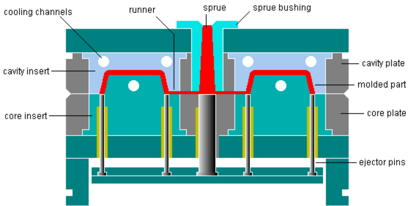
two- plate and two-cavity mold
