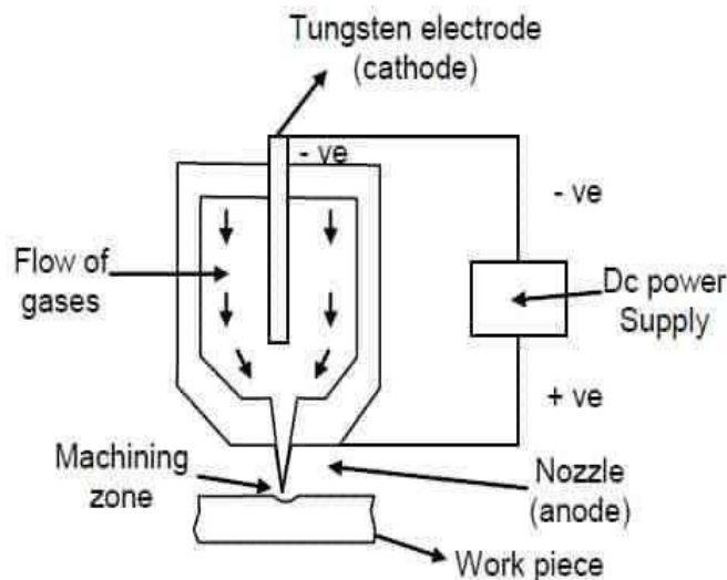
Figure Working Principle and Process Details of PAM
