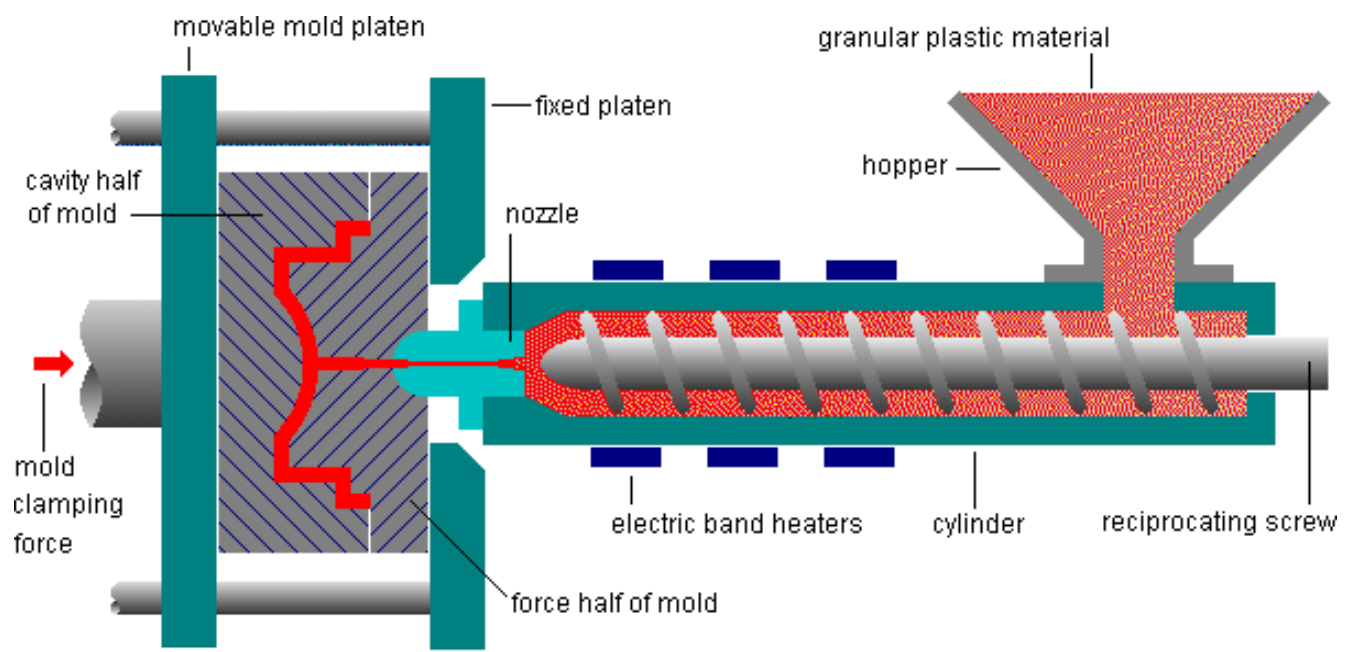
injection molding process
